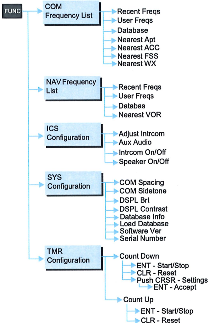
Functions Diagram
