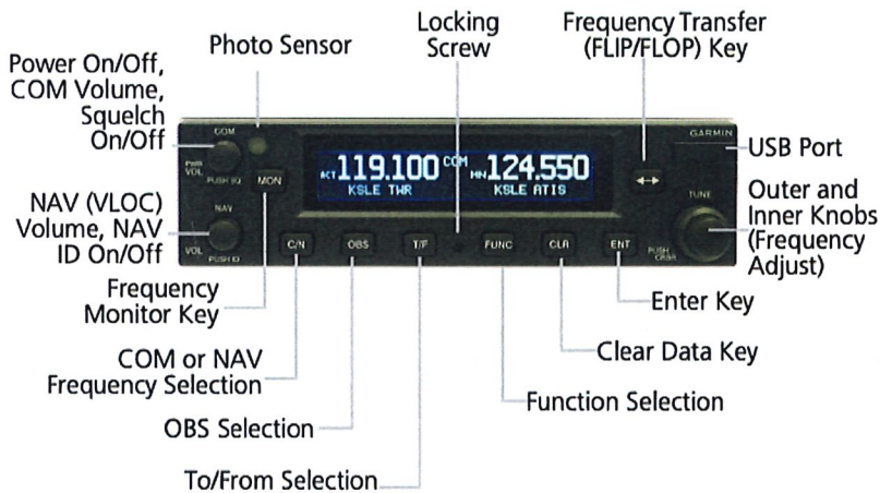
GNC 255 Front Panel Description
